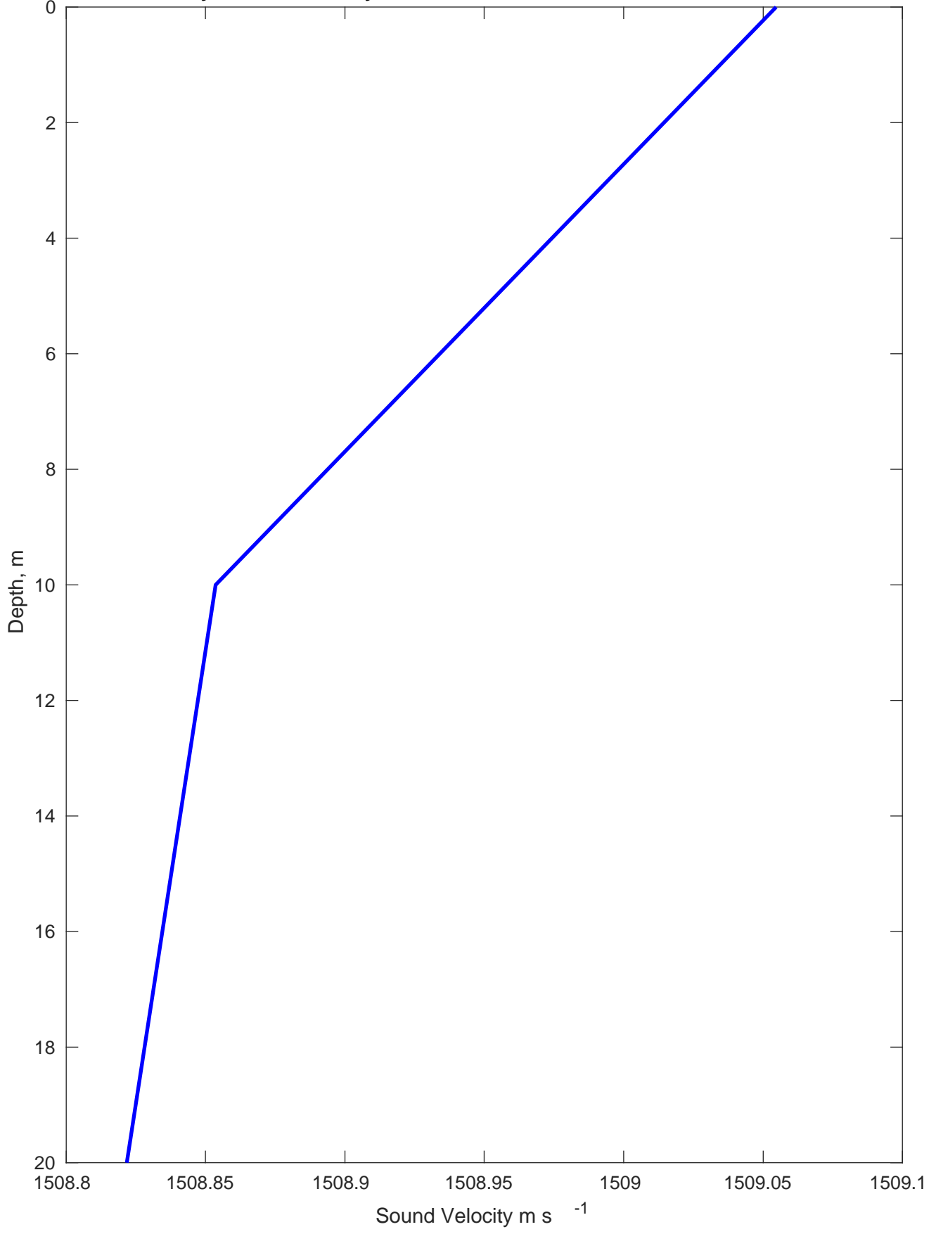
Sound Velocity Profile for Vineyard Wind GB14 on 13-Oct-2022 00:00:00
